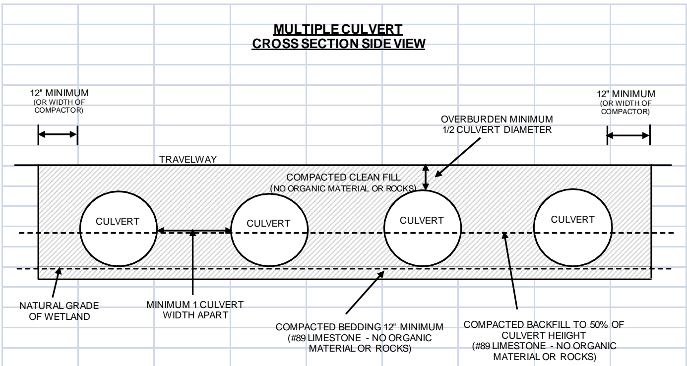
Figure 13. Typical culvert installation for multiple culverts, cross section side view.
