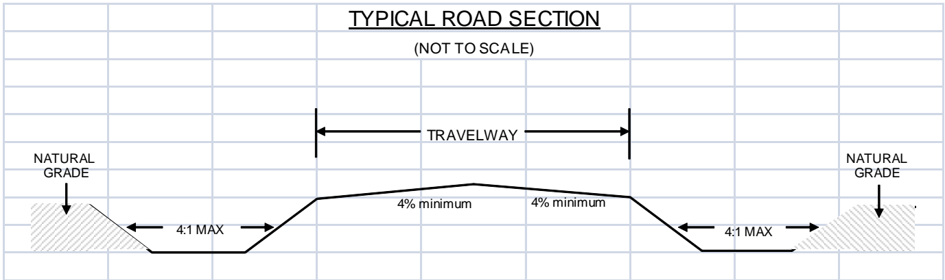
Figure 15. Typical Road Section Diagram.
