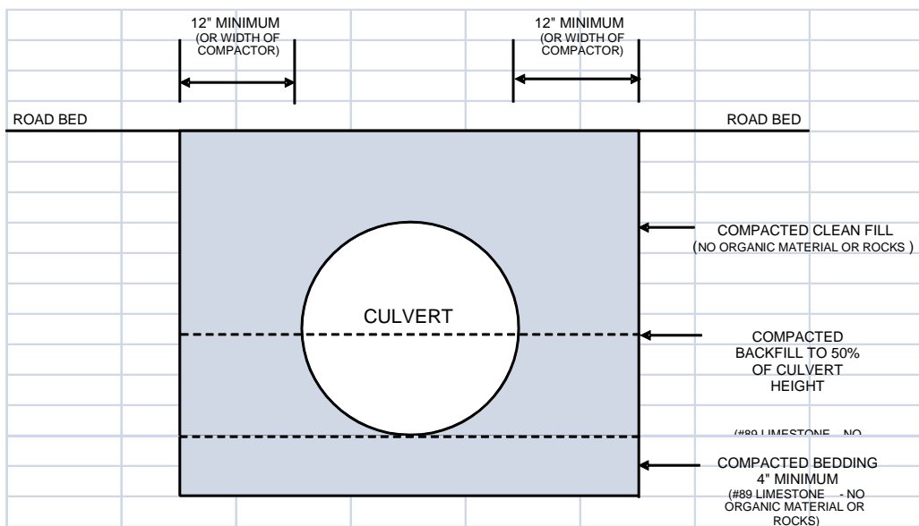
Figure 10. Typical culvert installation for single culvert, cross sectional side view.
