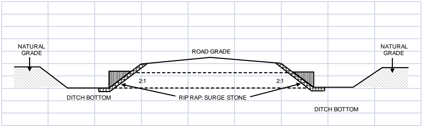
Figure 9. Typical culvert installation for single culvert, cross sectional side view.
