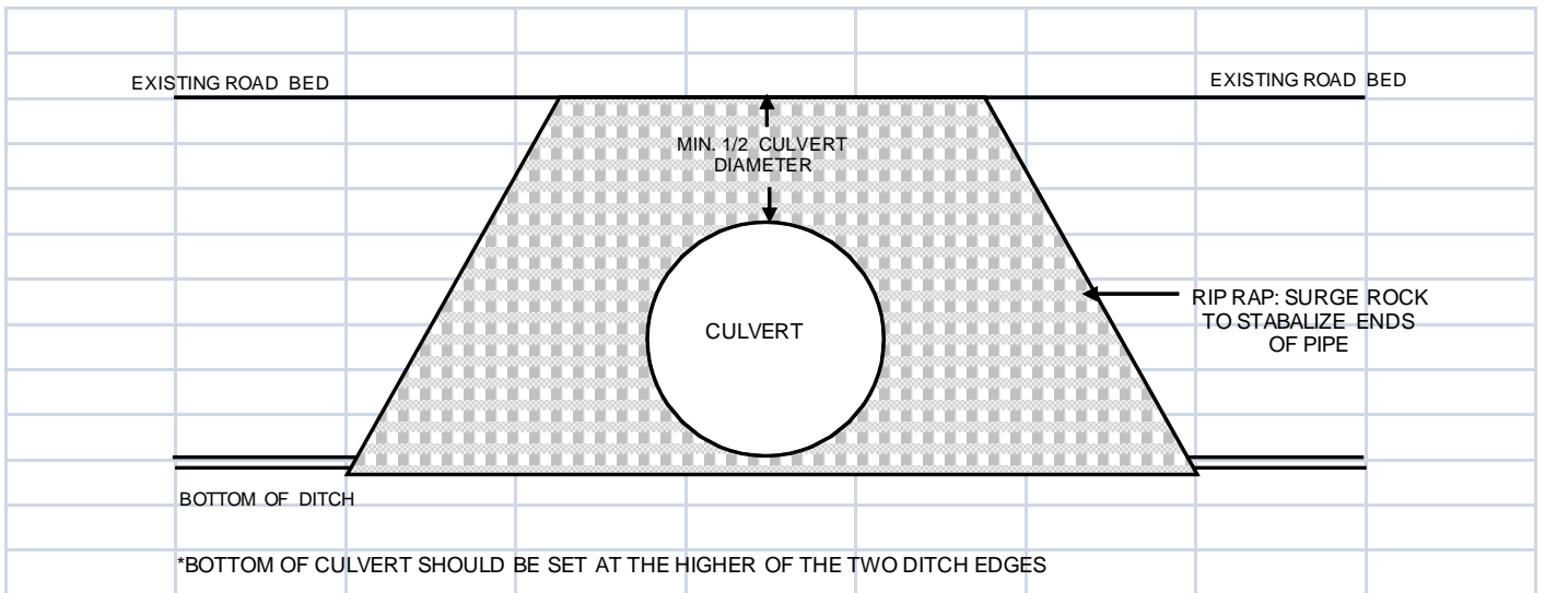
Figure 10. Typical culvert installation for single culvert, cross sectional side view.
