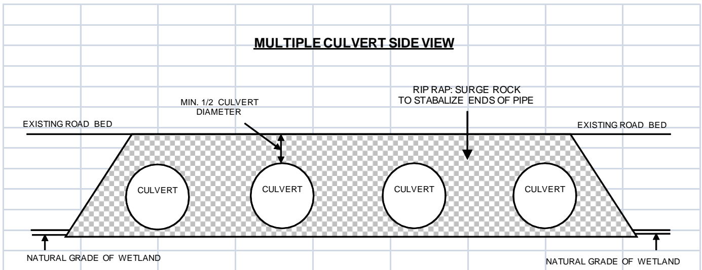
Figure 12. Typical culvert installation for multiple culverts, side view.
