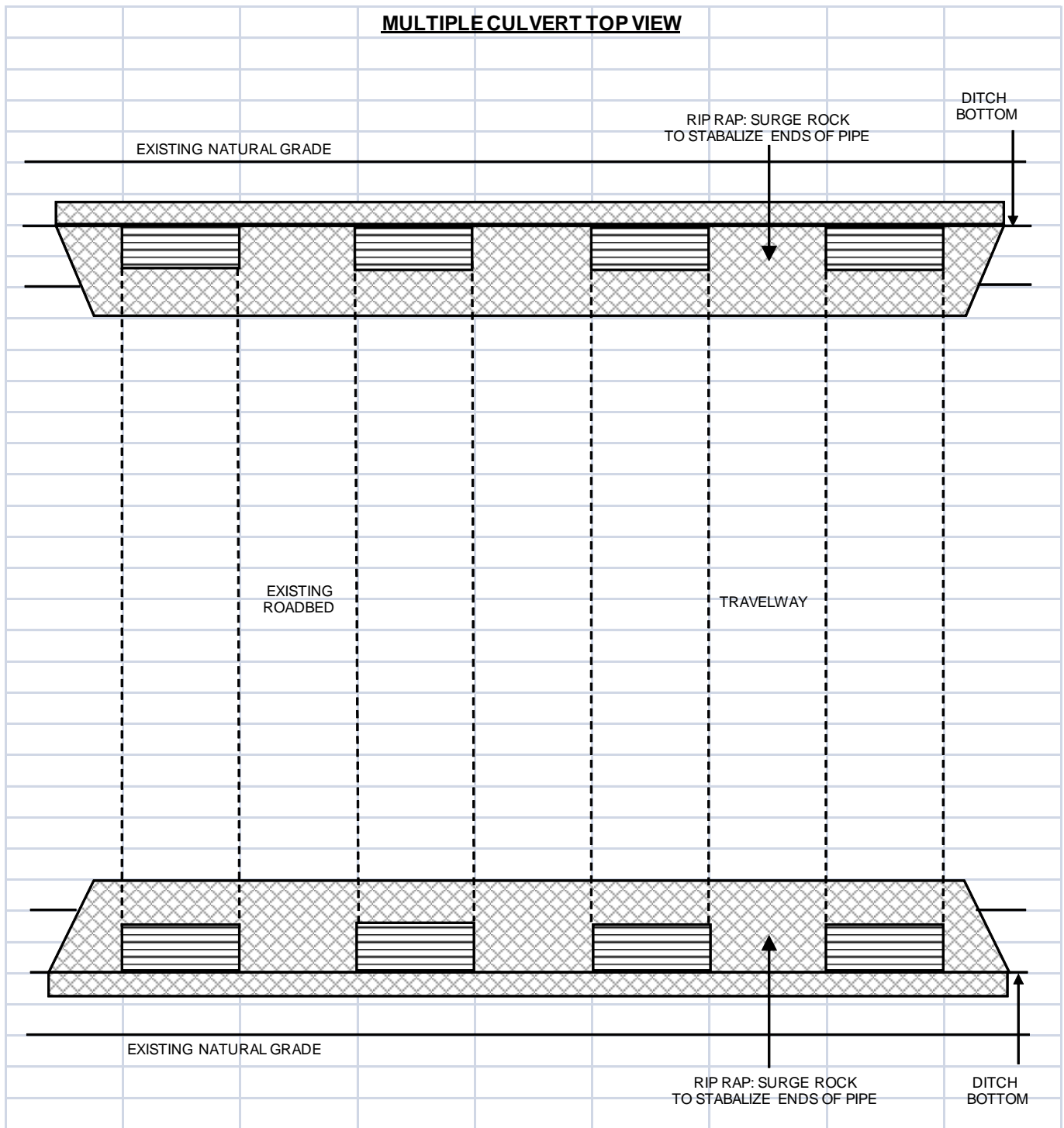
Figure 11. Typical culvert installation for multiple culverts, top view.
