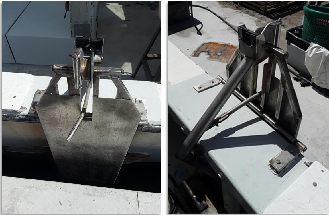
Example of Figure 3. Starboard side gunwale mounted trap tilt table with armature
