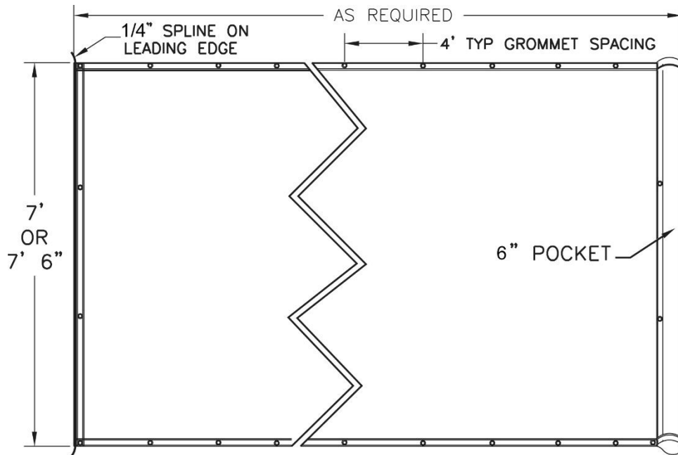
INDUSTRY STANDARD TARP DRAWING
