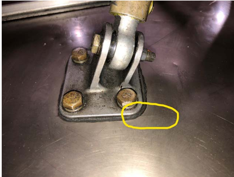
ENGINE DECK CRACK AT MOUNT
